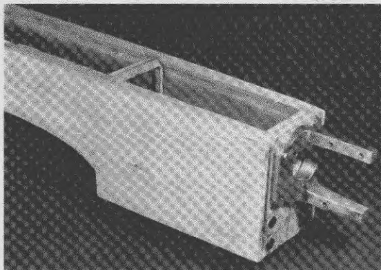
Above "basic box" with top to be added, but motor mount in place—and, below, the finished carved and sanded nose area—including nose-ring.
