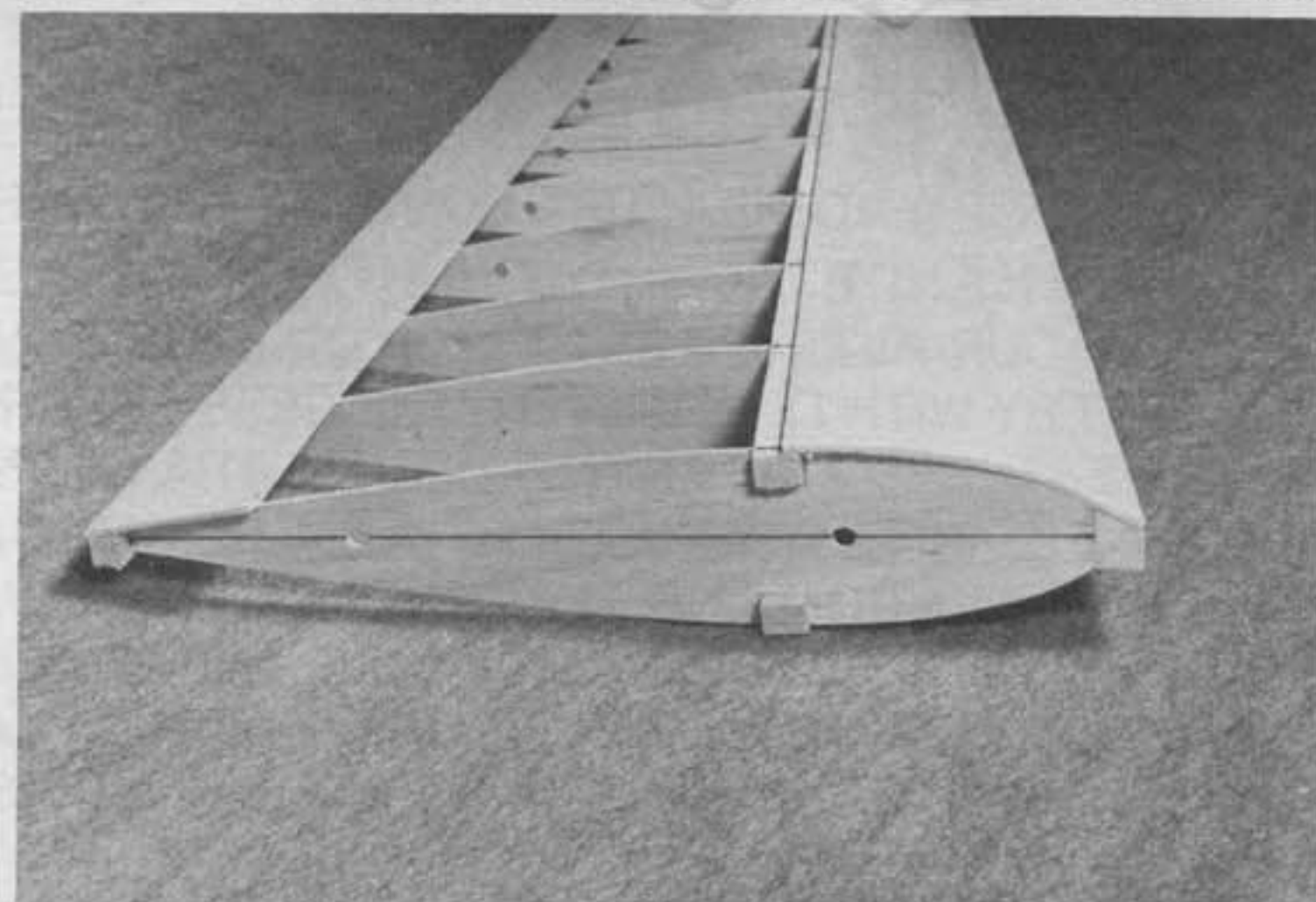
The T.E. and top L.E. sheeting installed.
