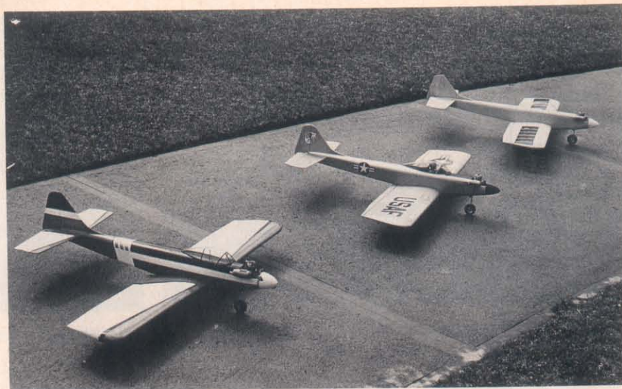
Don Dewey's original OS .25 powered New Era III in foreground. Lee Renaud's Veco-Lee .19 prototype in center, ready-to-cover proto at rear.
