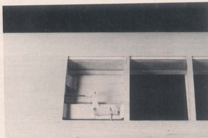
Aileron bellcrank. Note that link to horn is installed in middle hole.
